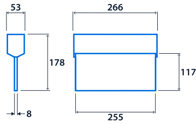
Ceiling Mounting
