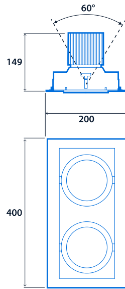
Cut-out - 380 x 182 Minimum ceiling void - 200
